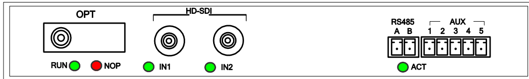
Figure 2-1-1 L-2SDI-FE-HD-TX Front Panel
